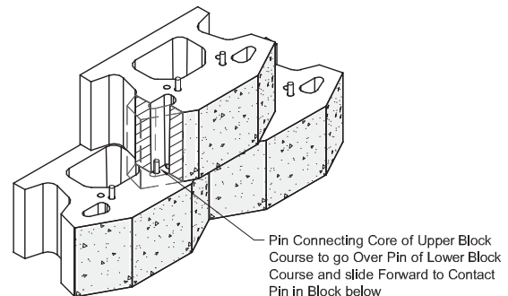
FIGURE F:1 - CONNECTION DIAGRAM
