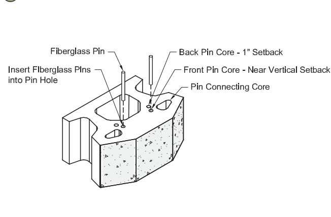
FIGURE E:1 - PIN INSTALLATION DIAGRAM
