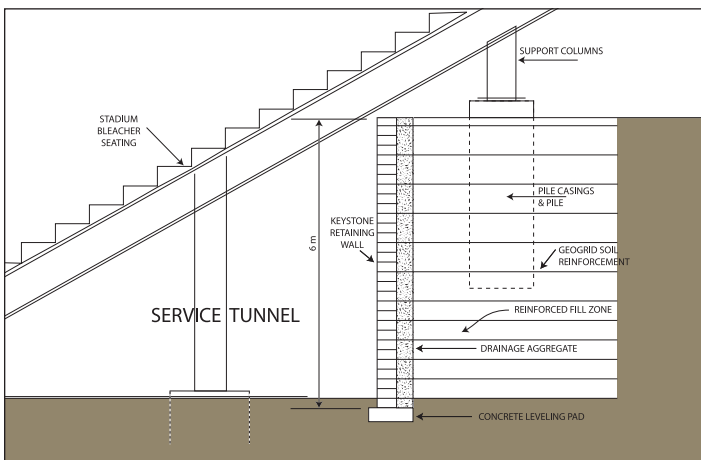
Typical cross section for service tunnel area
